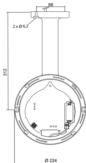
Double-sided bracket
