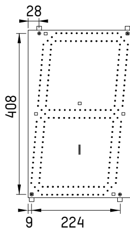
42-cm-LED-Modul
